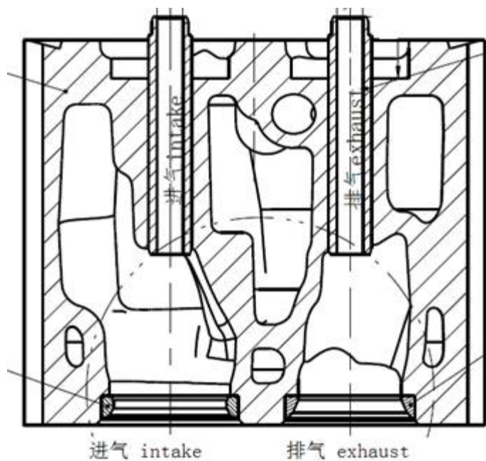
Cross-section of inlet and outlet port
