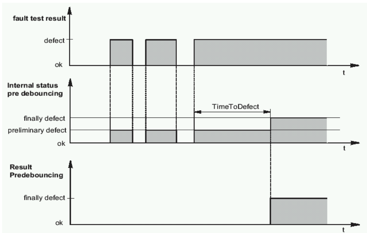
Fig 1 Fault test
